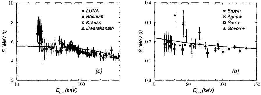
Fig. 2. Astrophysical S -factors for (a) the {}^3\text{He}({}^3\text{He}, 2p){}^4\text{He} and (b) the {}^3\text{H}({}^3\text{H}, 2n){}^4\text{He} reactions. The experimental data are taken from (a) Ref. [7] (filled circle, and filled triangle), Ref. [27] (open circle), Ref. [28] (open triangle) and (b) Ref. [29] (filled circle), Ref. [30] (cross), Ref. [31] (square), and Ref. [32] (triangle). The solid curves are our results.
