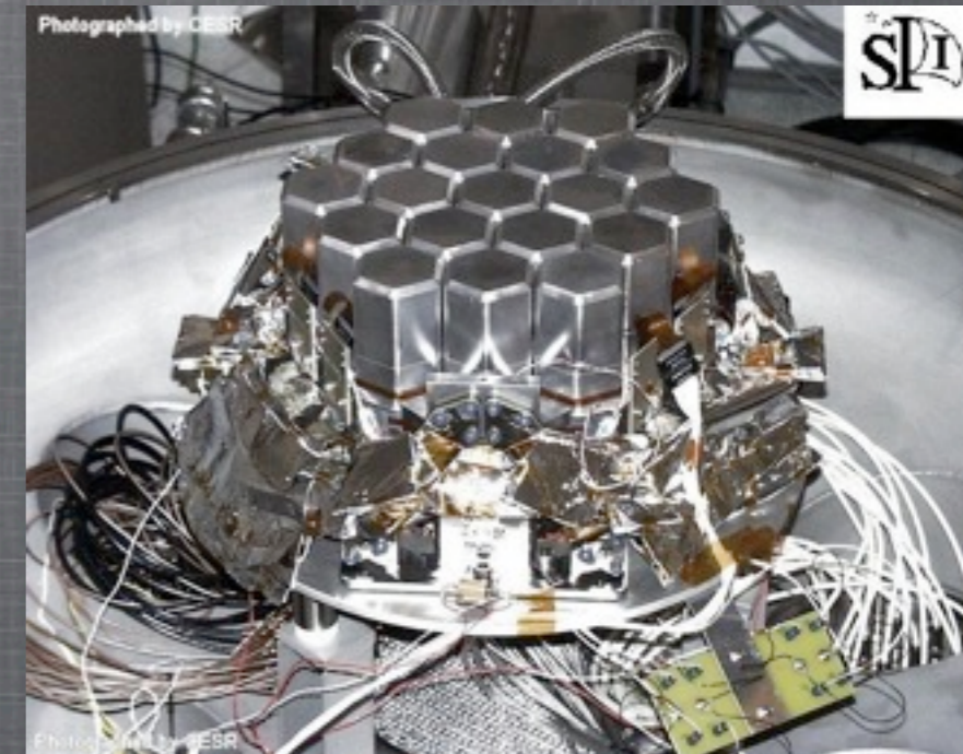
INTEGRAL's coded-mask spectrometer with a 19-element Germanium solid-state detector.
