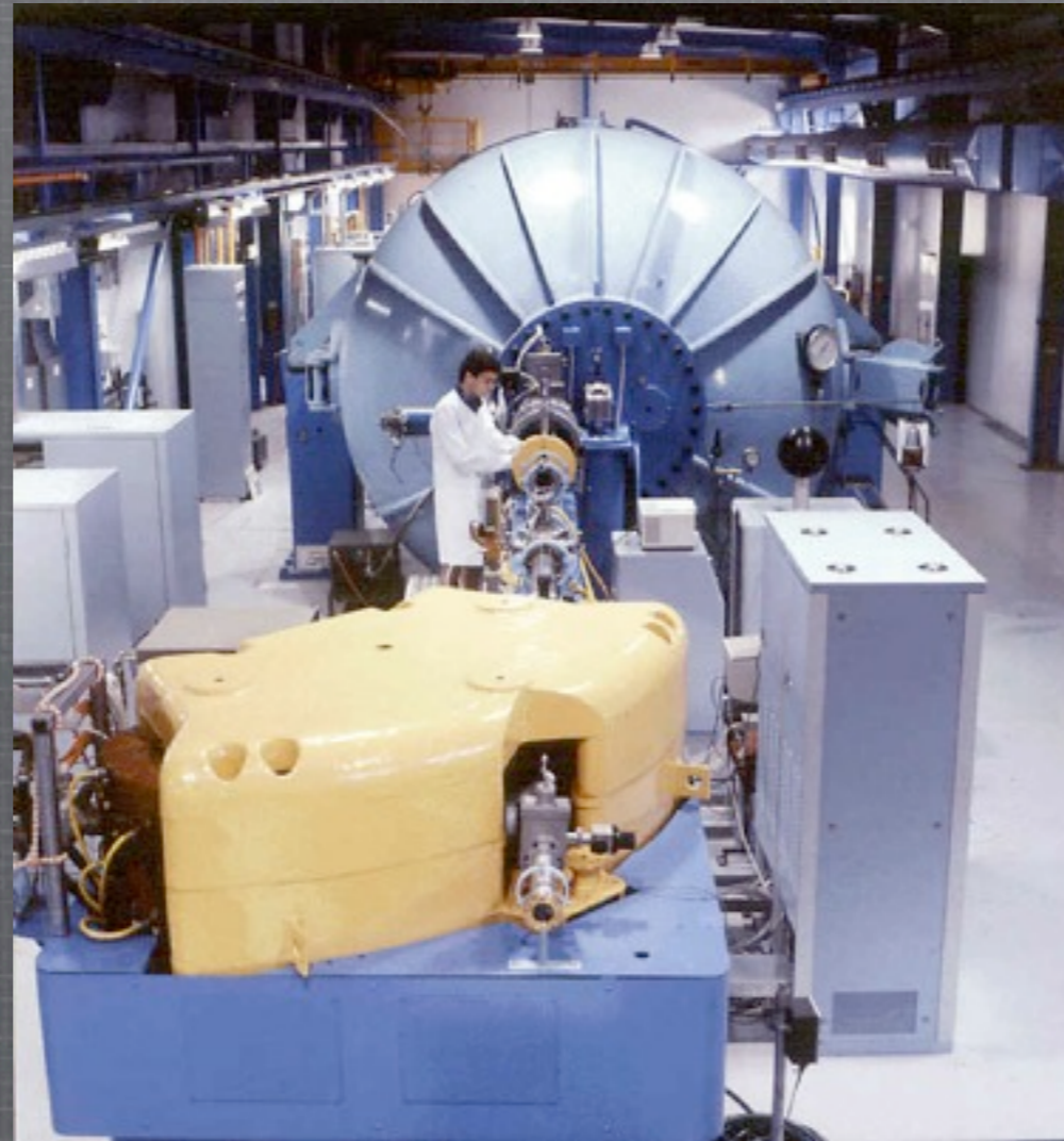
Accelerator mass spectrometer Institute for Environmental Research Australia
